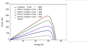
PV CURVE
