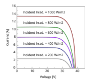
IV CURVE
